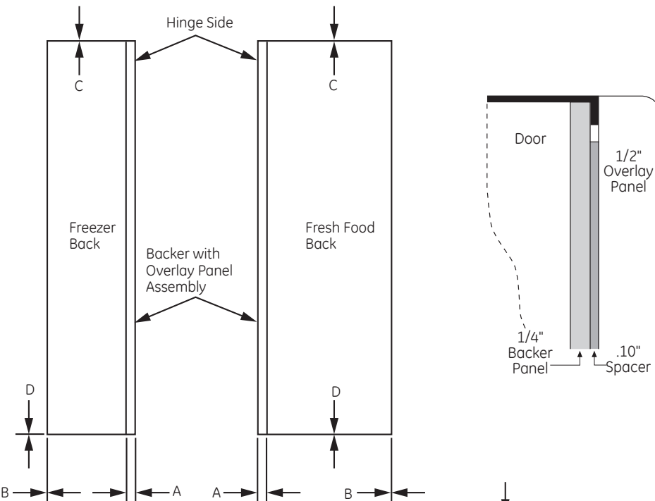
PANEL DIMENSIONS
