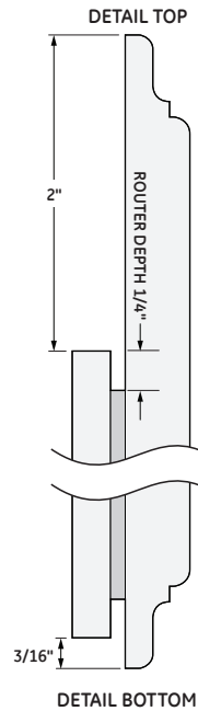
DETAIL BOTTOM
