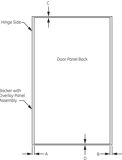
PANEL DIMENSIONS
