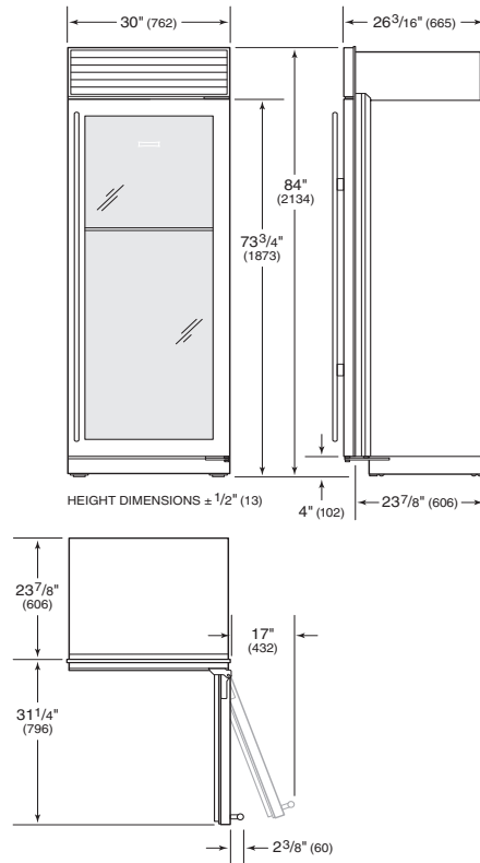
Dimensions based on stainless steel model. For flush inset, add 1/2" (13) to door clearance dimensions.
