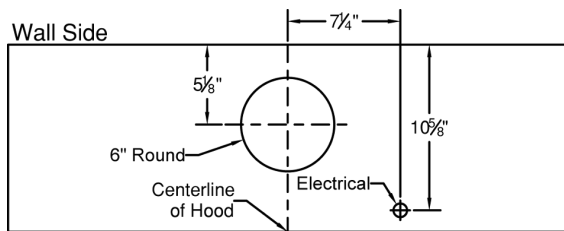
M600 &amp; M1200 Connection Diagrams
