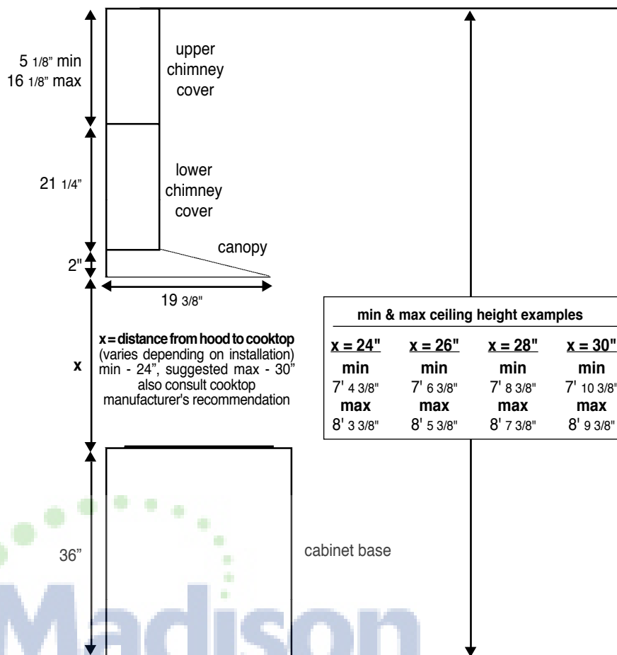
FIGURE 4A DUCTED INSTALLATIONS
