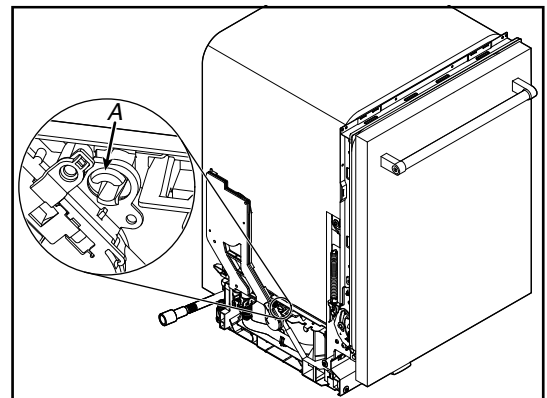
A. Plastic Retainer
