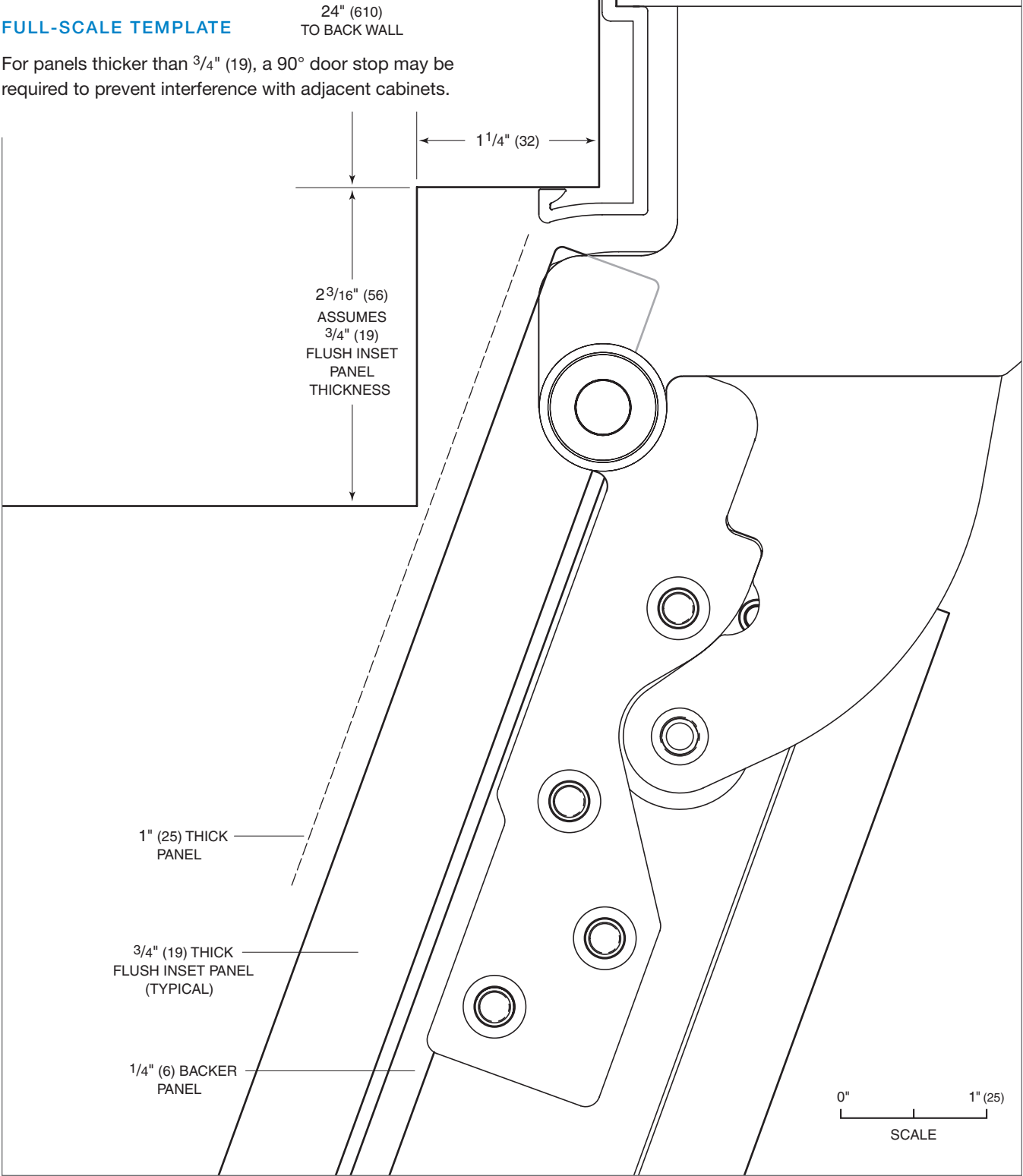
110° door opening (top view).
