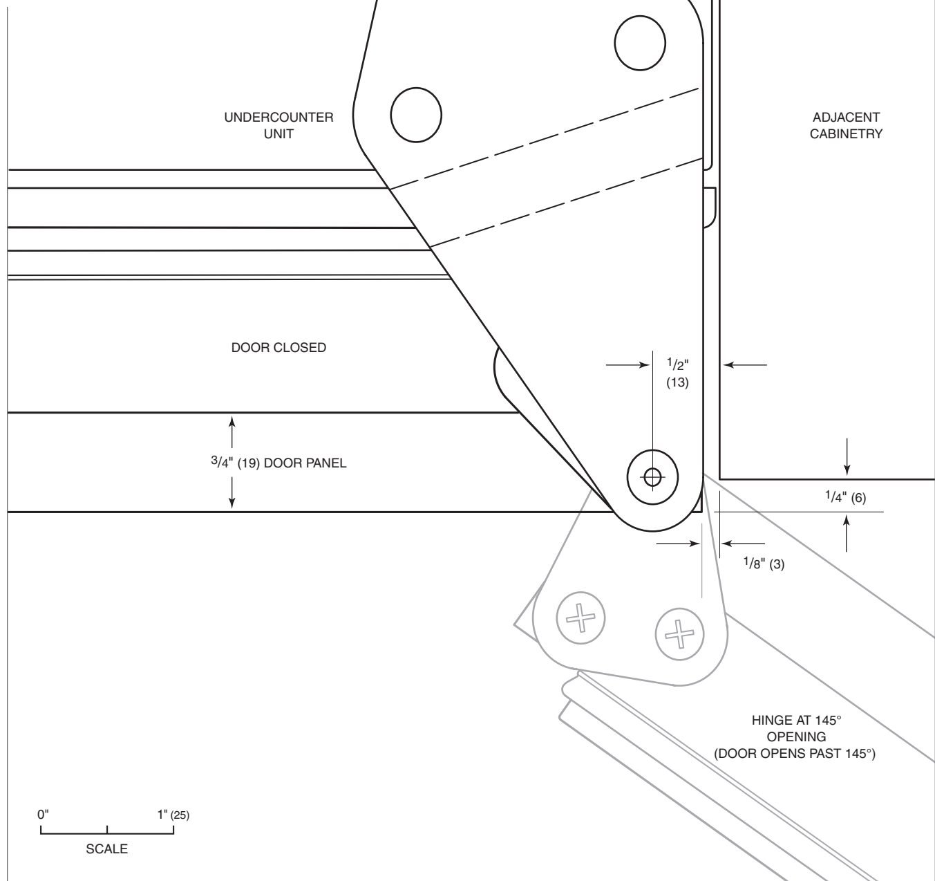
145° door opening (top view).
