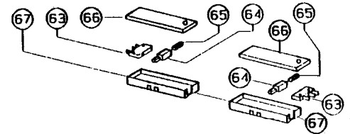
grease filter switch
