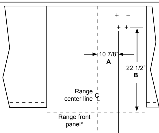
Bracket Placement
