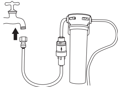
Diagram 3 Faucet connection
