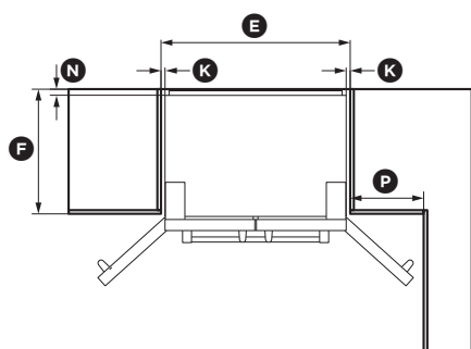
Flush with refrigerator chassis - full door rotation
