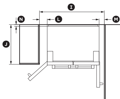
Flush with refrigerator door - 90° door rotation
