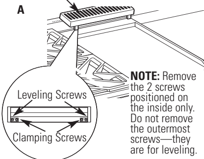
Griddle Flue Cover
