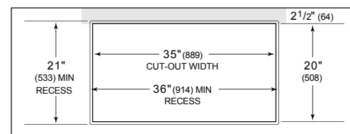
COUNTERTOP CUT-OUT
