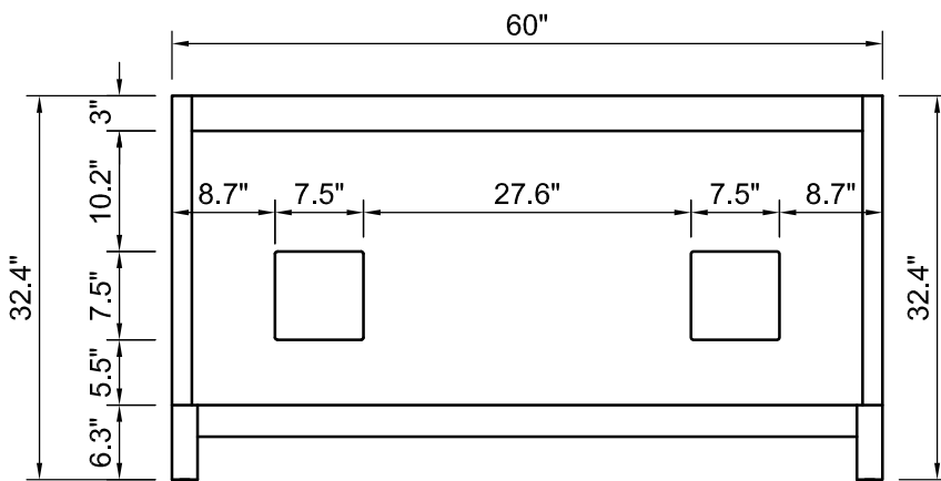
BACK VIEW
