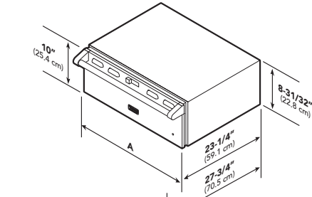
VEWD527/530/536 Custom Warming Drawer
