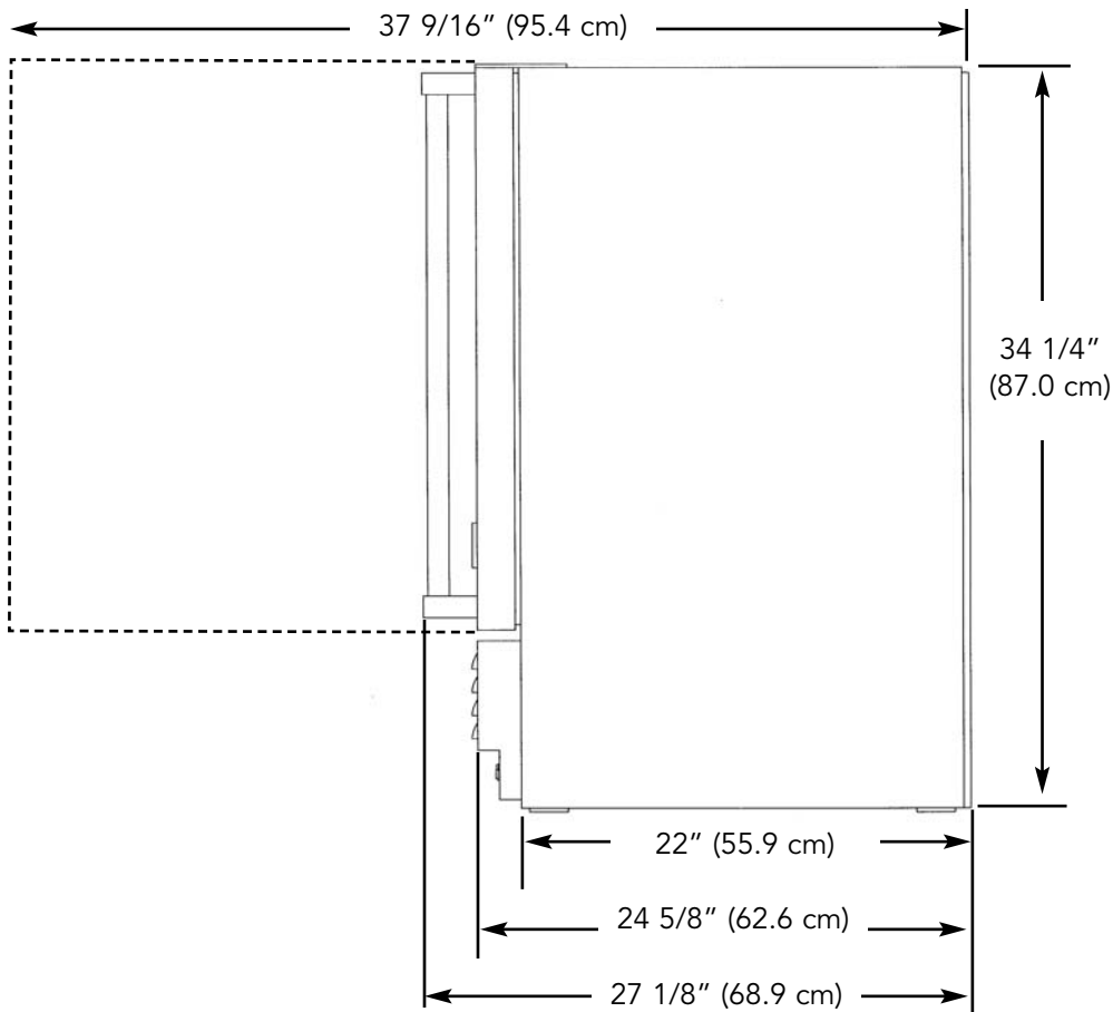
Side View
