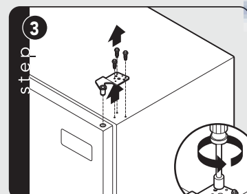
Unscrew 5/16" hex head screws from top hinge and remove hinge. Retain all screws for later use.
