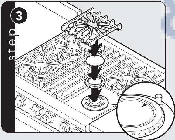
Burner caps are packed in styrofoam top pack with the grates. Place burner grate on top of burner cap and grate support. Note: Arrow on burner cap must be pointing towards back of range.
