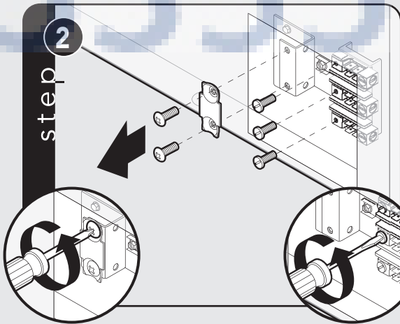
Remove supply cord strain relief bracket and three supply cord mounting screws on the terminal block.
