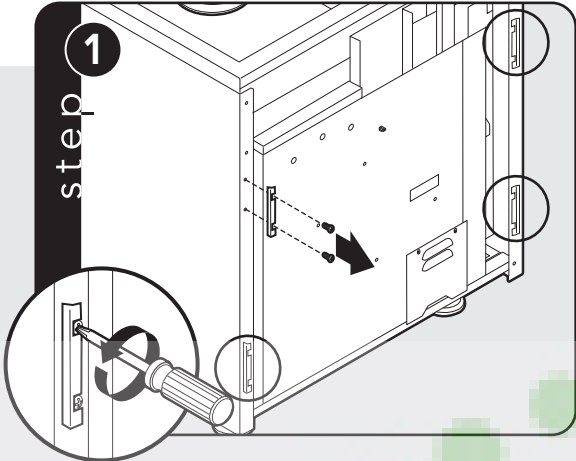
Unscrew four standoff brackets and remove.
