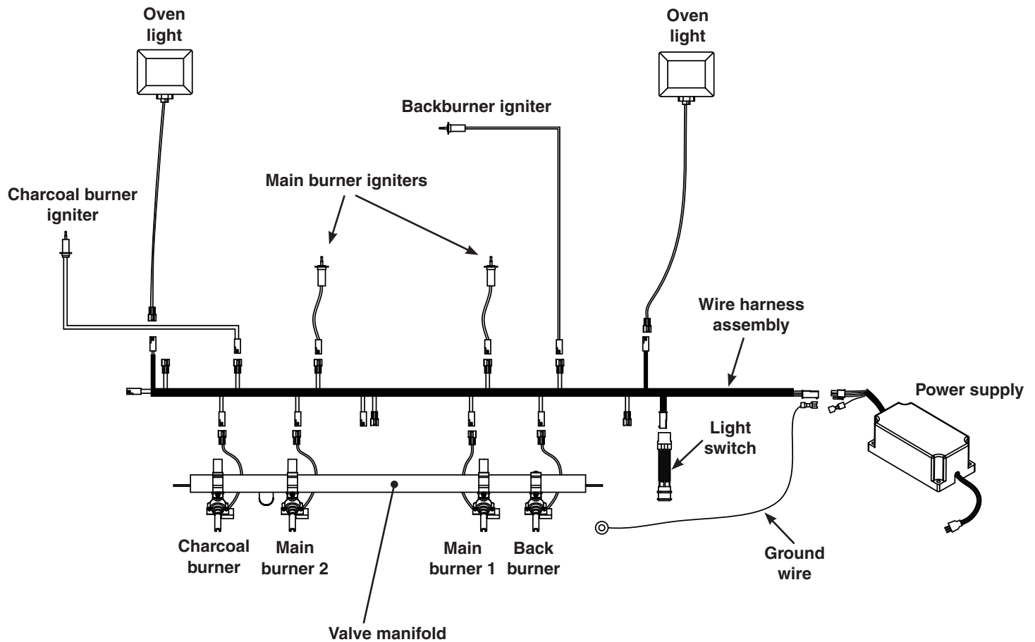
STAND-ALONE GRILL WIRING DIAGRAM *
