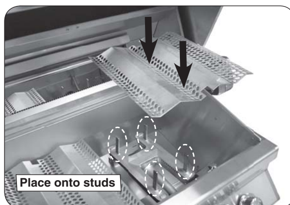
Fig. 16-2 Install flavor grids
