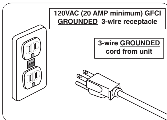
Fig. 16-3 Connect power cord
