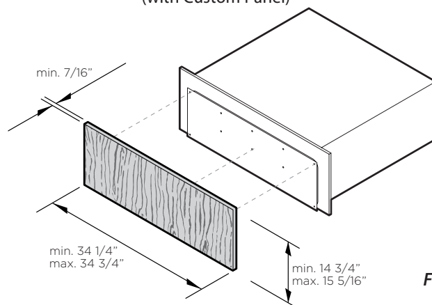
WDVI-30 DIMENSIONS (with Custom Panel)
