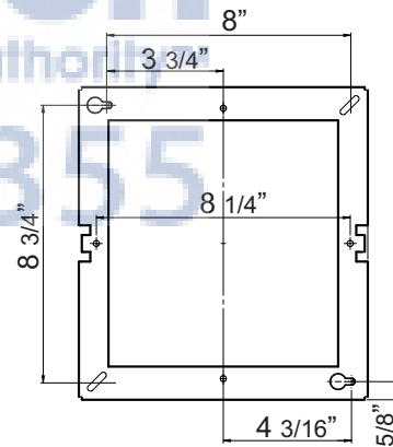
TOP SUPPORT FRAME (top view)
