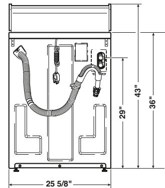
AWS76 (Shown on front) - 2-Speed Motor, 20 Cycles, 3 Water Temperatures, Extra Rinse, Fabric Selector Switch
