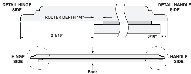
3/4" PANEL BOTTOM VIEW (AFTER ROUTING)
