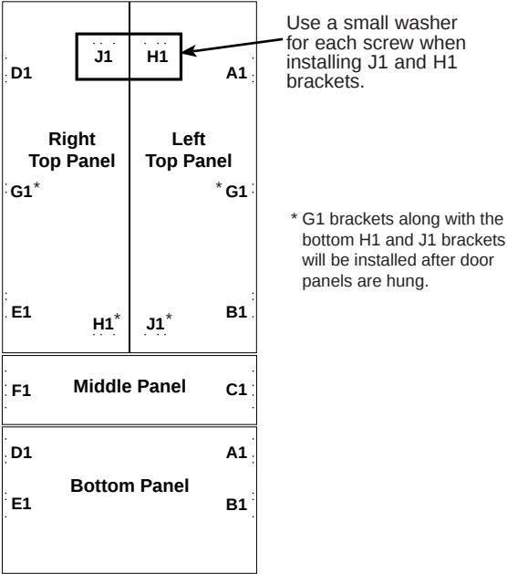
French Door Rear View of Panels
