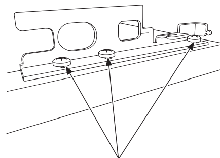
Single Door Rear View of Panels
