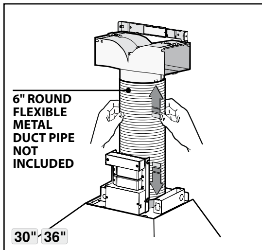
Fig.6: Once the air diverter has been inserted into the bracket and fastened to the wall connect the flexible (6" Round Metal) pipe to the diverter, use duct tape to seal.
