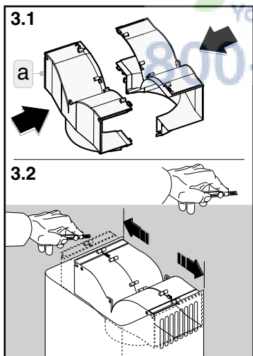
Fig.3: Put together the two parts of the air diverter as shown in picture no 3.1 . It may be necessary to cut the diverter to fit the width of the chimney as shown in picture 3.2 . A sharp blade or Hacksaw is recommended to trim the plastic.
