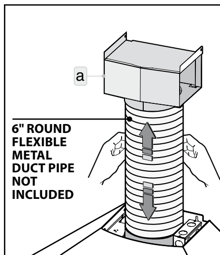
Fig.4: Once the air diverter has been inserted into the bracket and fastened to the wall connect the flexible (6" Round Metal) pipe to the diverter, use duct tape to seal.
