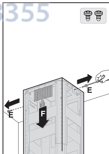
Fig.2: To remove the two screws E , to take down the lower chimney F .
