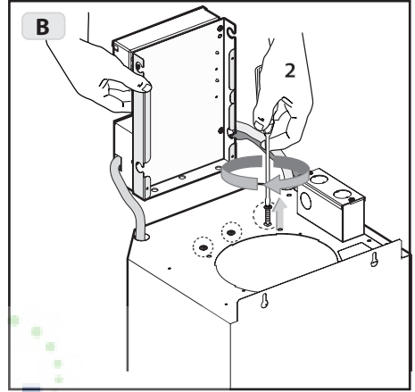
Fig.14B: Remove the 3 fixed screws.
