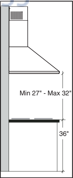
› Mounting height and clearance:
