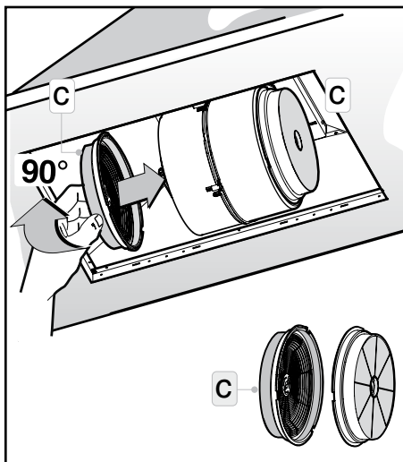
Fig.8: The filters C must be applied to the suction unit inside the hood, centering them inside of it and turning them 90° until they snap into place.
