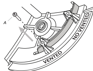
A. Venting method screw
