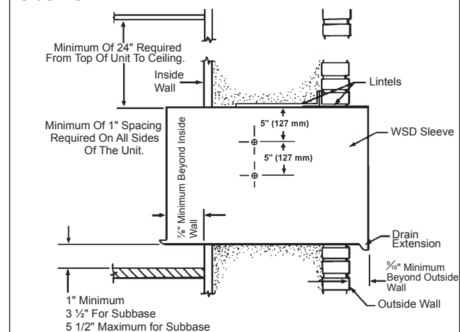
Figure 7 Side View
