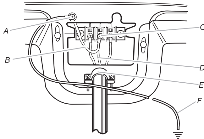
A. External ground conductor screw B. Neutral ground wire C. Center, silver-colored terminal block screw
