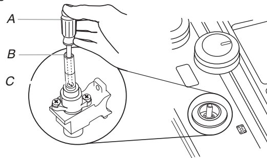
A. \frac{3}{32} " (#0 [2.0 mm]) flat-blade screwdriver (screwdriver shaft must be a minimum of 2" [5.1 cm] long)
