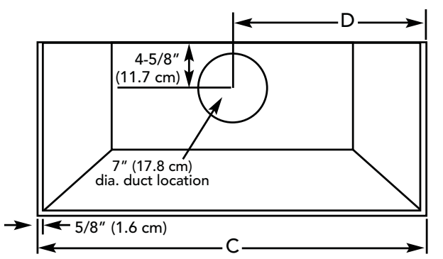
300 or 600 CFM Interior Ventilator Installation 36", 42" W. Models
