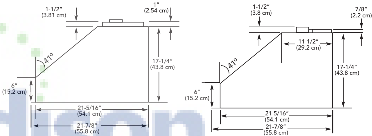
For 900, 1200 or 1500 CFM Exterior or In-Line Ventilator Installation
