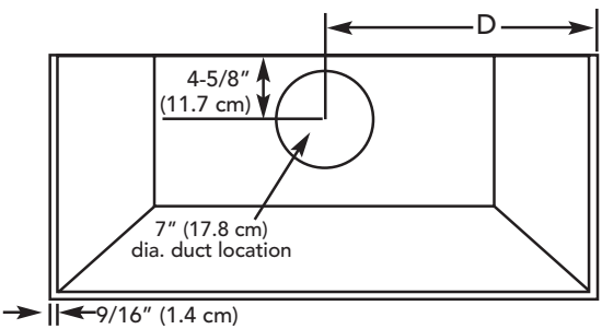
300 or 600 CFM Interior Ventilator Installation 36", 42" W. Models
