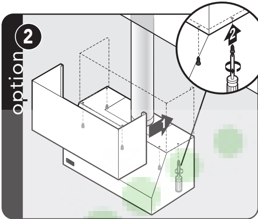
Slide the duct cover in place and fasten from inside canopy using the sheet metal screws provided.
