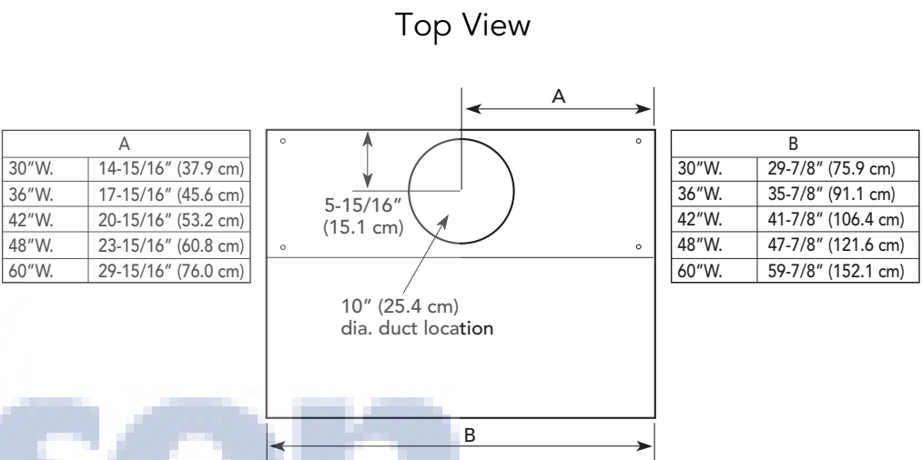
900 or 1200 CFM Exterior or In-Line Ventilator Installation for all
