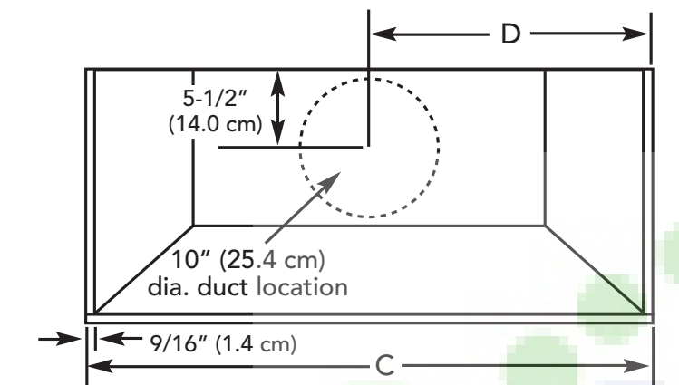
1200 or 1500 CFM Exterior or In-Line Ventilator Installation 48", 60" W. Models
