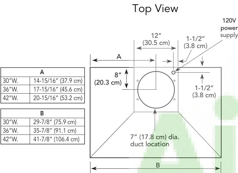
300 or 600 CFM Interior Ventilator Installation for 30", 36", & 42" models
