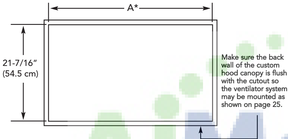
Custom Hood Canopy Bottom Cutout Dimensions
