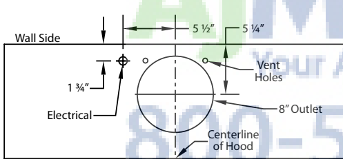
600 CFM B200 Dual Blower (Top View)
