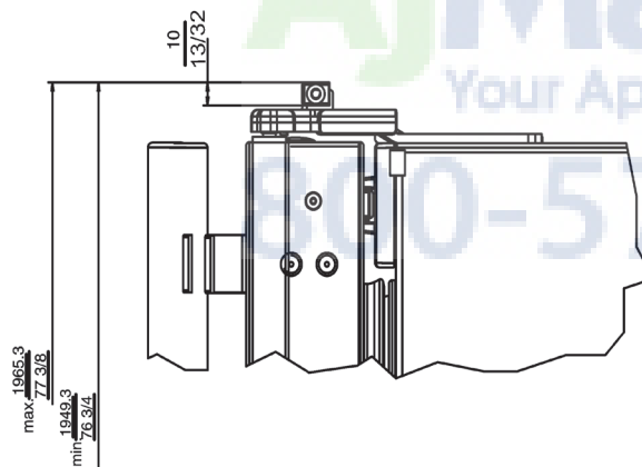
Side view right without ventilation grille
