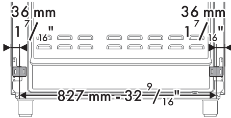
(Rear view)
