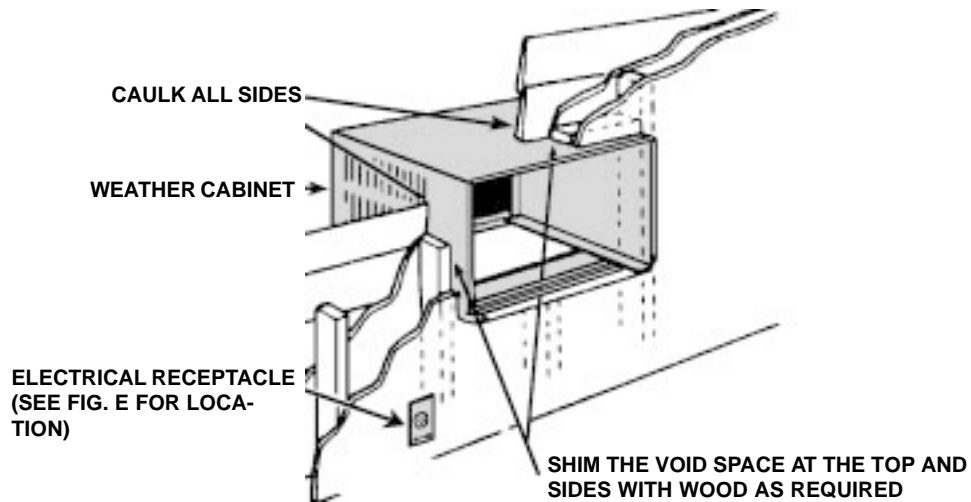
FIGURE C FRAME WALL CONSTRUCTION
