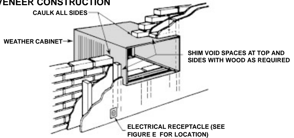
FIGURE D BRICK VENEER CONSTRUCTION
