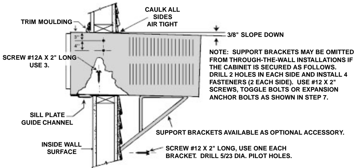
FIGURE F TYPICAL INSTALLATION
