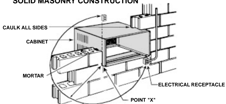
FIGURE E SOLID MASONRY CONSTRUCTION
