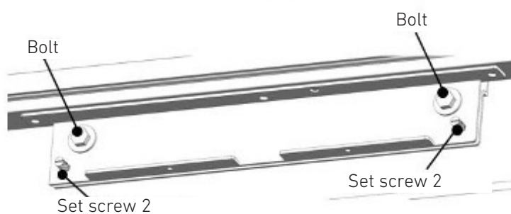
Panel-Adjustment Mechanisms
