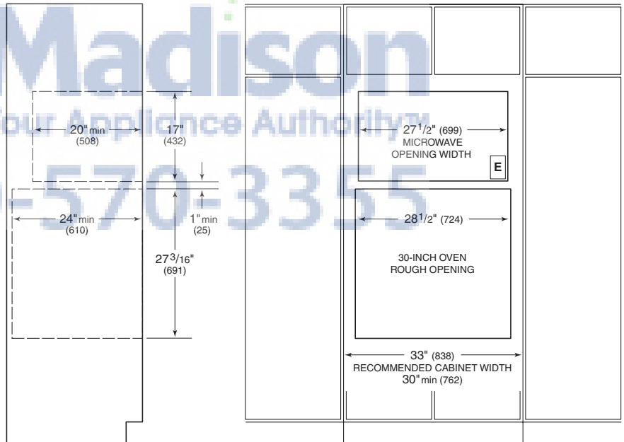
Installation with 30" L Series trim
