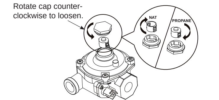
Regulator style B
