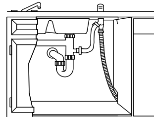
Waste Tee Installation Figure HH
