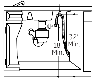
Disposer Installation
