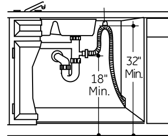
Waste Tee Installation Figure II
