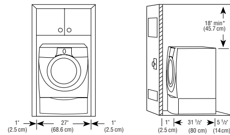
Recessed or Closet Installation with Pedestal
