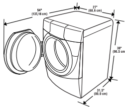
Installation with Stack Kit #8519492
