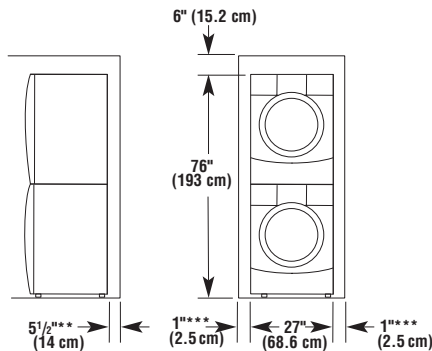
Installation with Stack Kit #8519492
