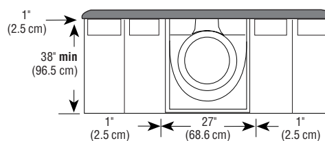
Custom Undercounter Installation
