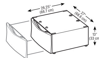
Optional Storage Drawer (Pedestal) Part No. LAB2700M
