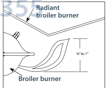
Fig. 19 Typical section of proper flame
