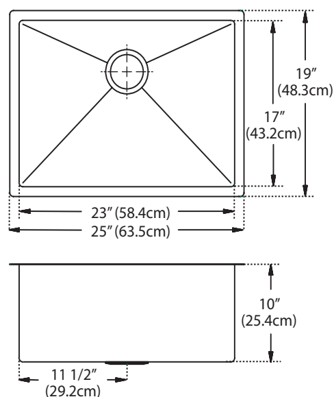
Dimensional Drawing
