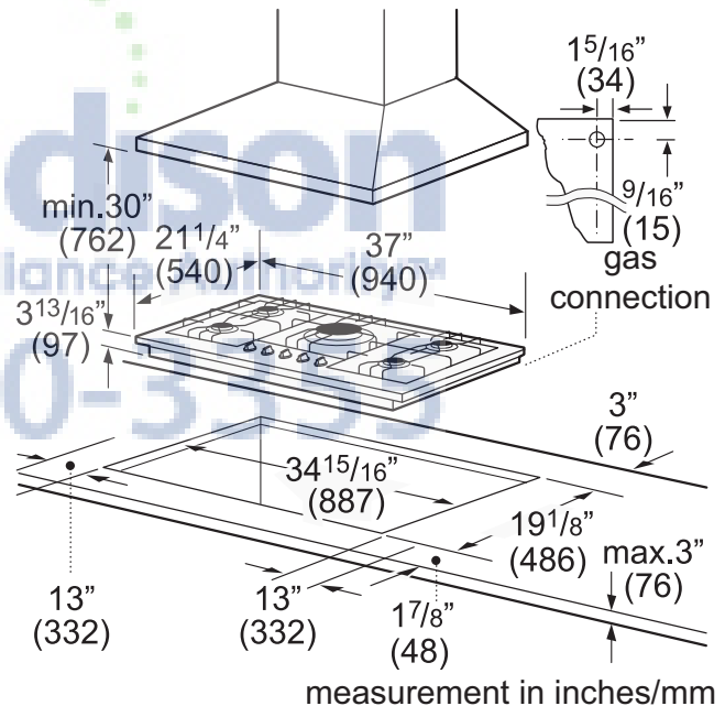
Figure 2: Cutout Dimensions
