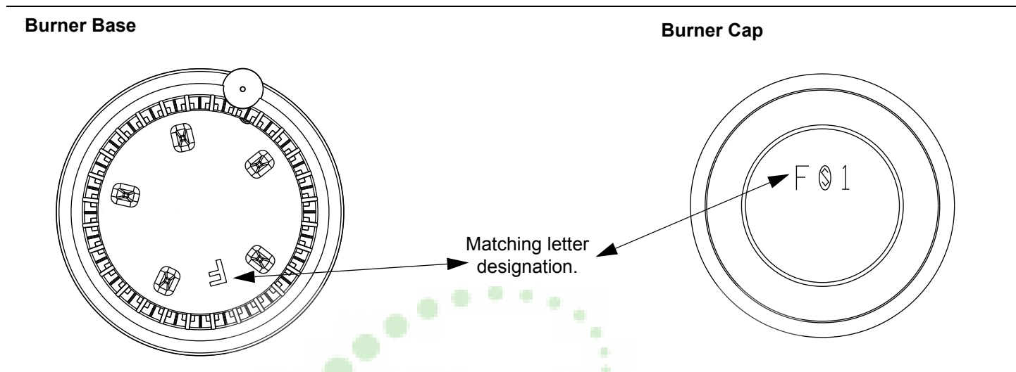
Figure 4: Burners Caps
