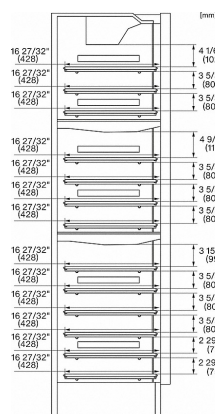
KWT2602Vi/SF, KWT2612Vi/SF, KWT2601Vi/SF, KWT2611Vi/SF, inner space, MasterCool, installation drawings
