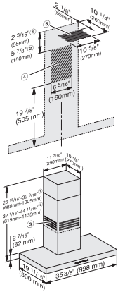
PUR98W, DAP1927 (Installation drawing) – USA/CDN
