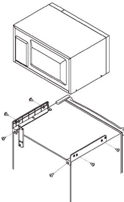
MicroFridge® with Safe Plug® Assembly Diagram - Model 2.5MF4RE
